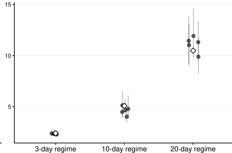
Generation-time SD
